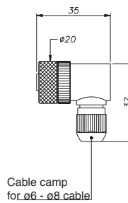
CON041 CON042 IP67
