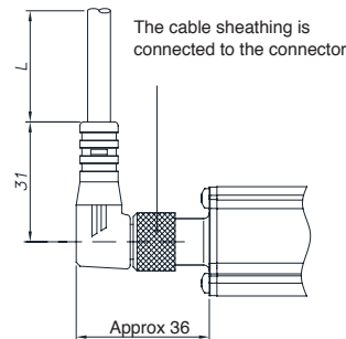
PRE-ASSEMBLED CABLE WITH 90° CONNECTOR
